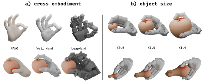
Fig. 5. Augmentation across object scales and dexterous hand embodiments without per-case retuning.
