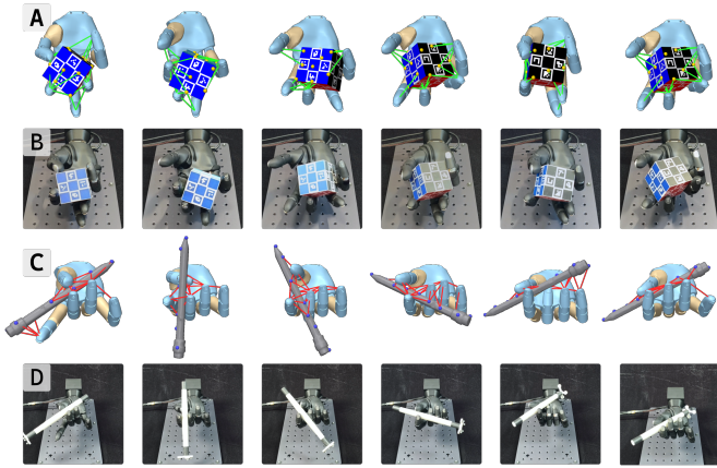
Fig. 4. Interaction-mesh visualizations of retargeted reference trajectories (A,C) and corresponding zero-shot real-world executions (B,D) for cube reorientation and pen spinning on the Wuji Hand.
