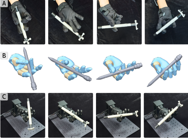
Fig. 1. TOPORETARGET converts human hand-object trajectories collected with a motion-capture glove (A) into robot references for contact-rich dexterous manipulation. These retargeted references are used to train RL policies that execute dexterous skills in simulation (B) and transfer zero-shot to Wuji Hand (C).
